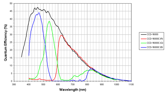
Spectral sensitivity
